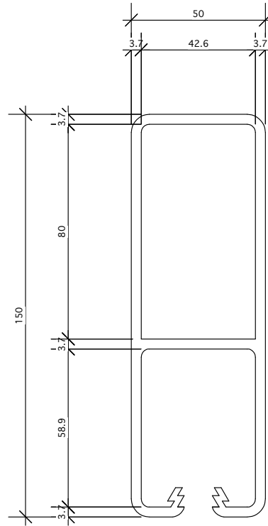
PROPOSED MULLION SECTION SCALE 1:2 @ A4
