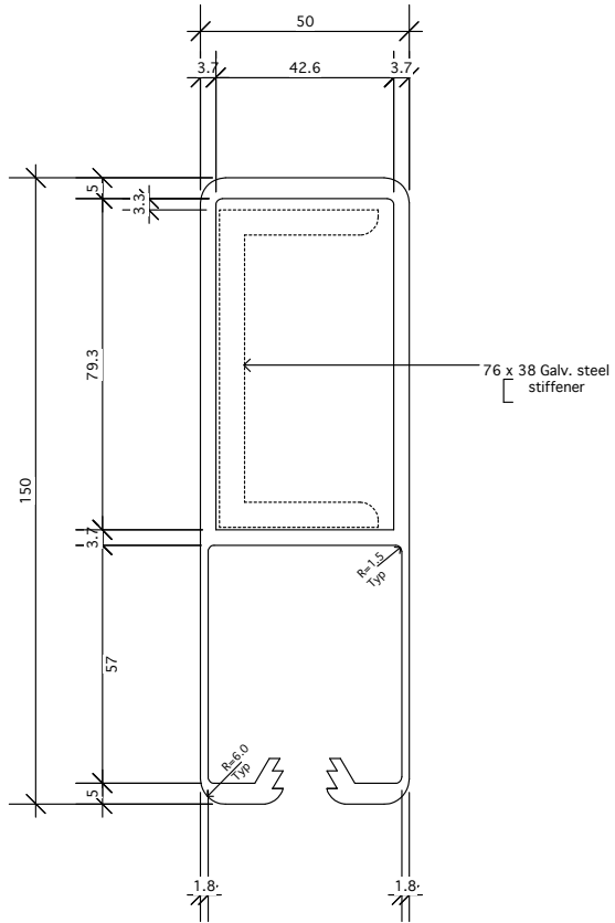
PROPOSED MULLION SECTION SCALE 1:2 @ A4
