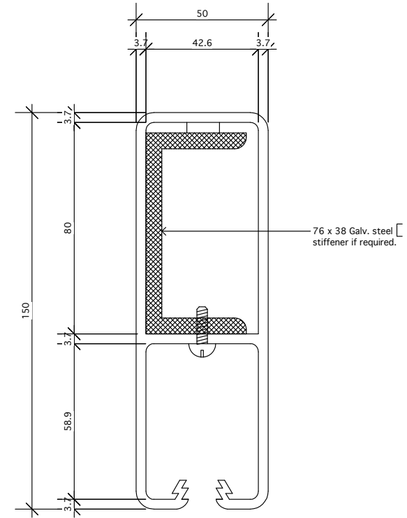
PROPOSED MULLION SECTION WITH STIFFENER SCALE 1:2 @ A4
