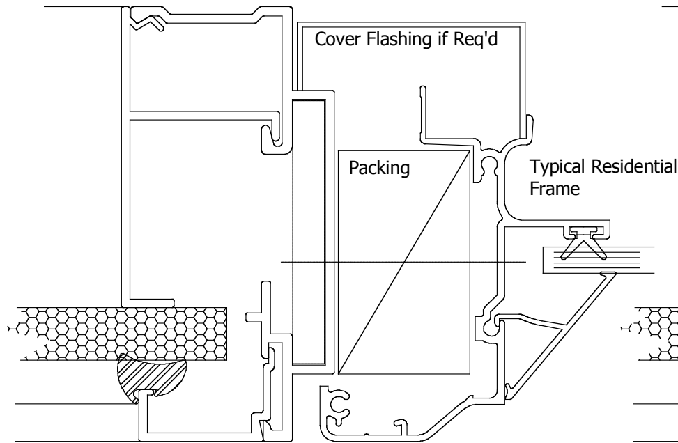
5 WINDOW JUNCTION
