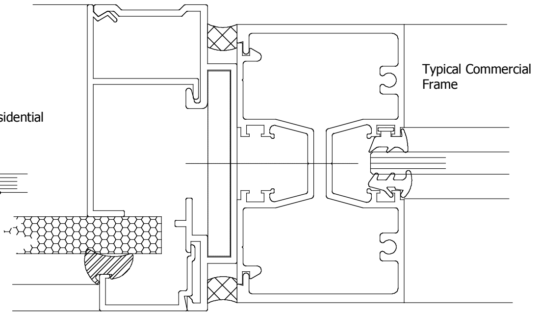
6 WINDOW JUNCTION
