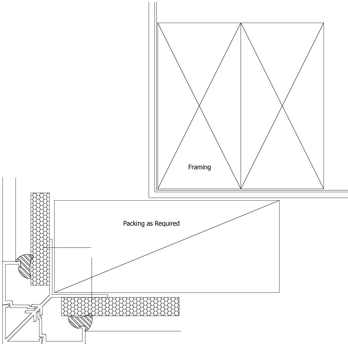
8 EXTERNAL CORNER
