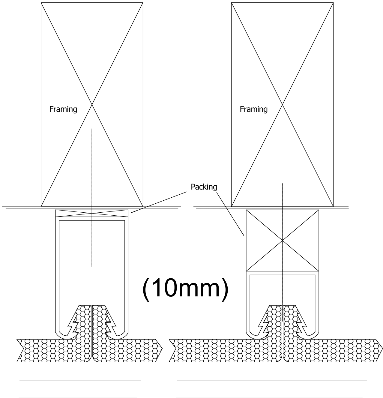
④ CONNECTOR
